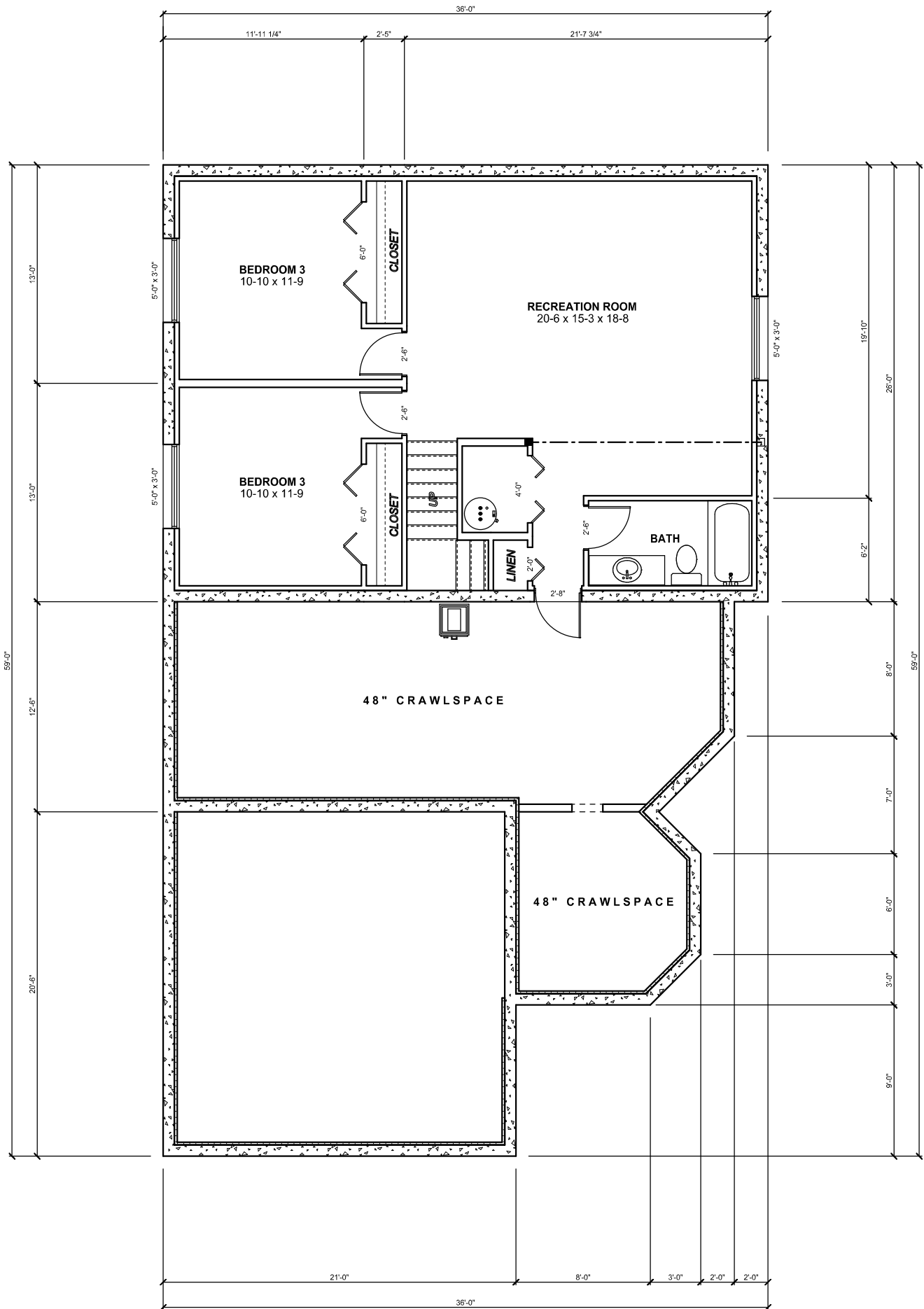
BASEMENT PLAN BASEMENT AREA: 936 sq.ft. CRAWLSPACE AREA: 541 sq.ft.
