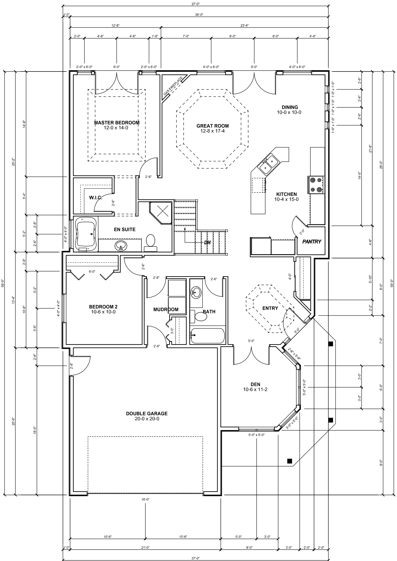
MAIN FLOOR PLAN MAIN FLOOR LIVING AREA: 1473 sq.ft. GARAGE AREA: 440 sq.ft.
